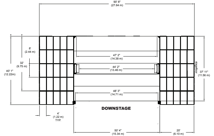
Floor View with Covered Wings
