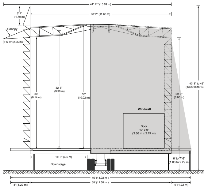
Side View with Extension Platforms
