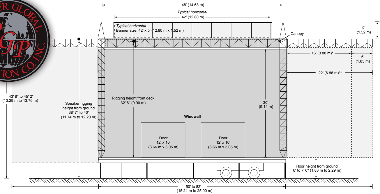
Front View with Windwall & Banner
